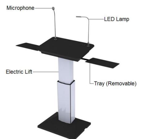
MSS-02B (Aluminum)
